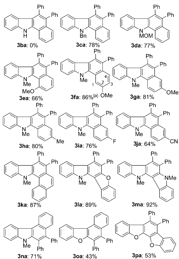
Scheme 2. Palladium-catalyzed cycloaromatization of 1 with alkyne 2a . Standard reaction conditions: 1 (0.20 mmol), 2a (0.30 mmol), Pd(OAc) 2 (0.02 mmol), K 2 CO 3 (0.06 mmol), TBAB (0.10 mmol), PivOH (0.20 mmol), DMF (2 mL), 100 °C, O 2 (1 atm), 12 h. Yields are of isolated products. [a] 2-OMe/4-OMe = 56:44, the ratio of the regioisomers was determined by 1 H NMR spectroscopy. Bn = benzyl, MOM = methoxymethyl.
