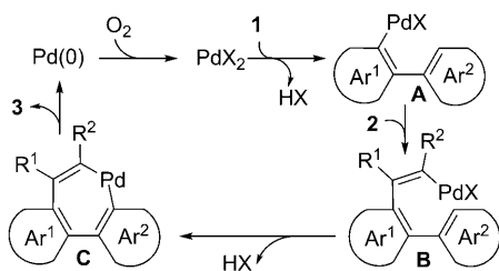
Scheme 3. Plausible mechanism for the reaction of 1 with 2 .
