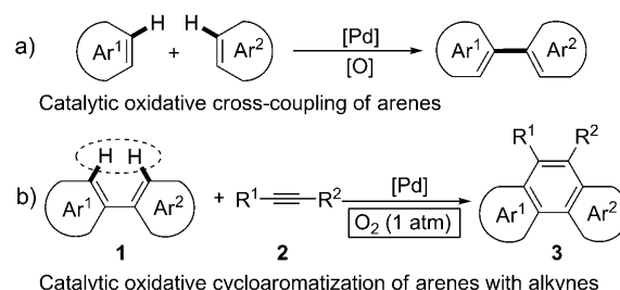
Scheme 1. a) Direct cross-coupling between two arenes. b) Cycloaromatization reaction through the activation of C–H bonds between biaryls and alkynes.
